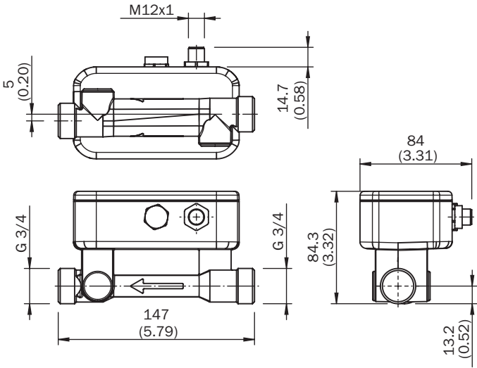
Plan coté DN 15, G 3/4
