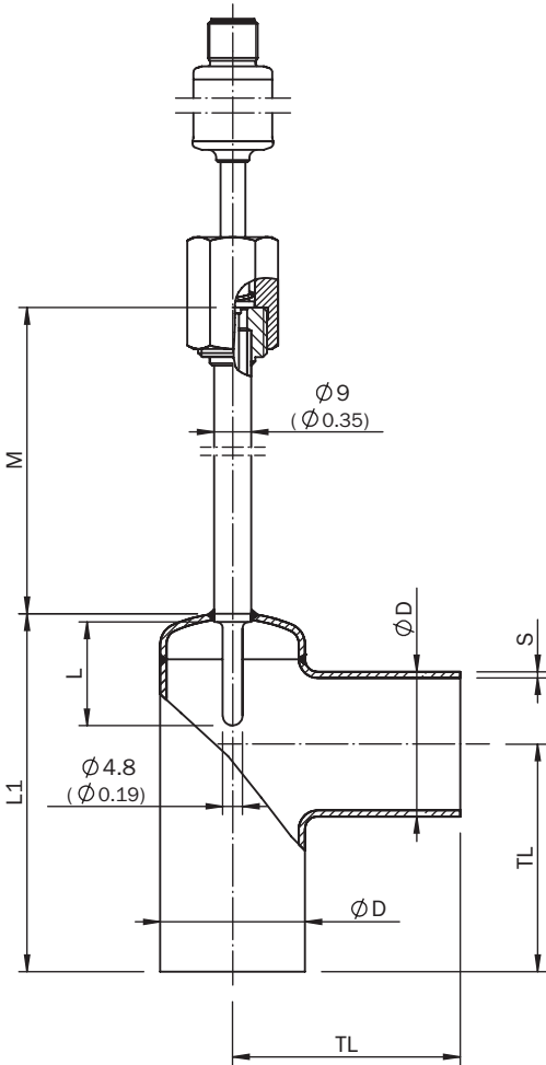
Complete assembly
