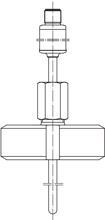
Complete assembly
