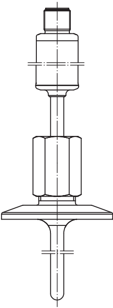
Complete assembly
