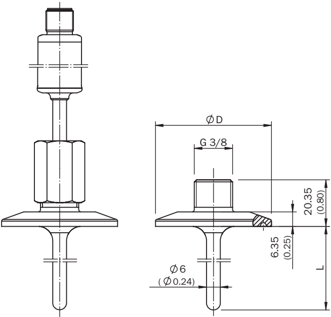
Complete assembly
