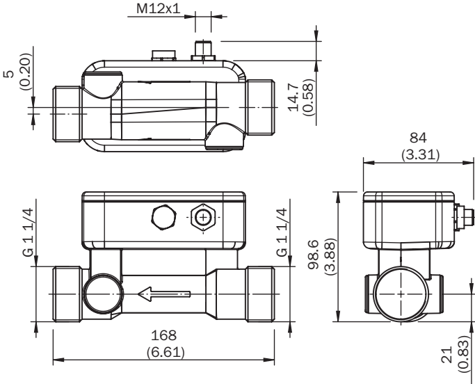
Plan coté DN 25, G 1¼
