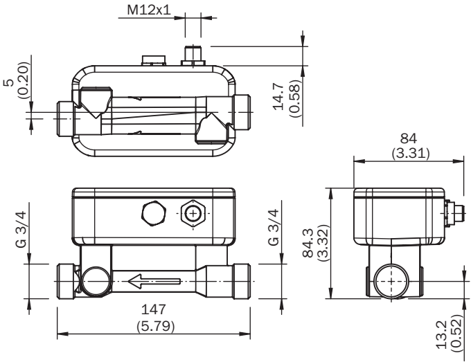
Plan coté DN 15, G 3/4
