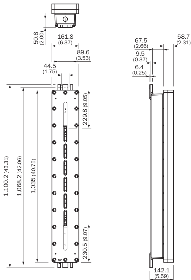
Plan coté deTec4 Core Ex, 600 mm
