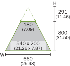
TriSpector1060 Typ. field of view in mm (inch)
