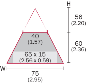
TriSpector1008 Typ. field of view in mm (inch)
