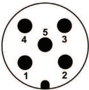
View to the connector M12 fitted to the encoder body
