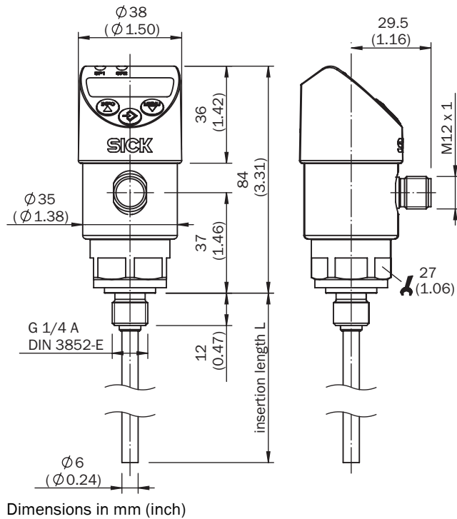
Dimensional drawing TBS with connection G 1/4 A according to DIN 3852-E
