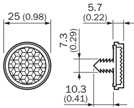
Dimensions in mm (inch)
