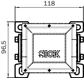
Dimensions in mm (inch)
