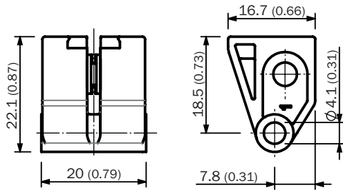
Dimensions in mm (inch)
