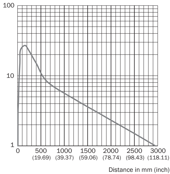
Characteristic curve typ. max. on reflector PL20A (measured in preferred direction)
