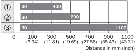
Sensing range diagram WTB11-2, 1,100 mm
