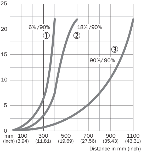
Characteristic curve WTB11-2, 1,100 mm
