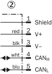
② Stecker M12, 5-polig
