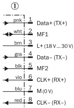
① Stecker M16, 8-polig
