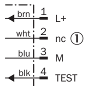
Sender
