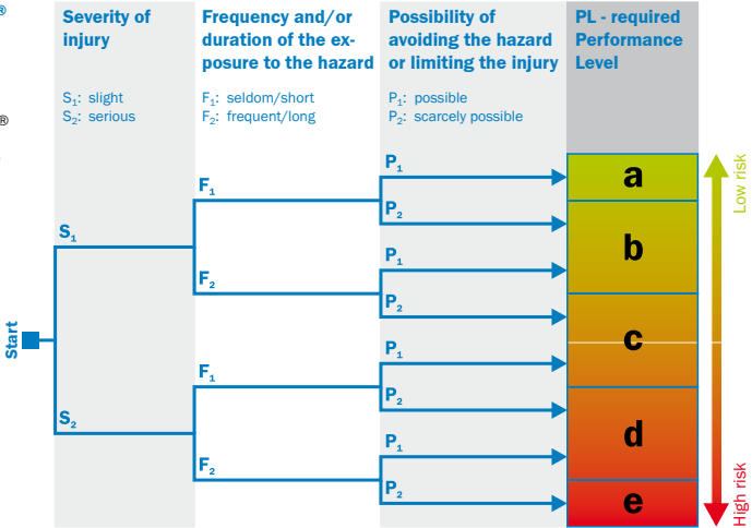
Performance Level according to EN 13849-1
